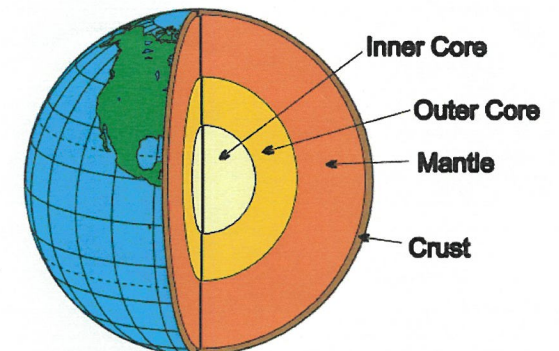
Layers of the Earth
